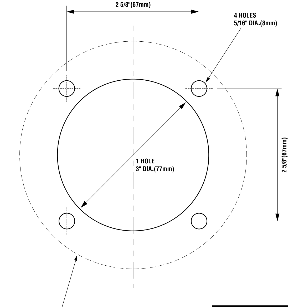
HELM FLANGE OUTLINE (for reference only) 4 1/2" (115mm) DIA. MAXIMUM COVERAGE
